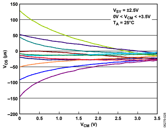
Figure 27. Input Offset Voltage vs. Common-Mode Voltage
