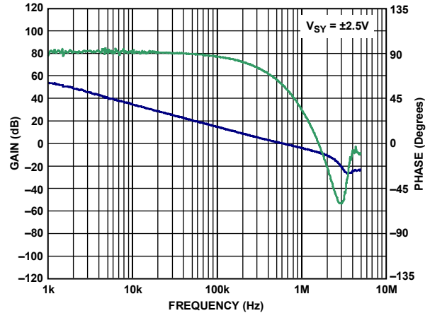
Figure 28. Open-Loop Gain and Phase Shift vs. Frequency
